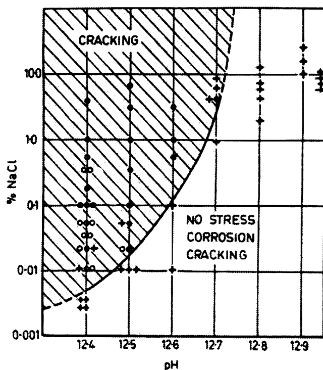
Fig. 3.3—Stress corrosion crack resistance as a function of pH and chloride content (Klotz 1969).
