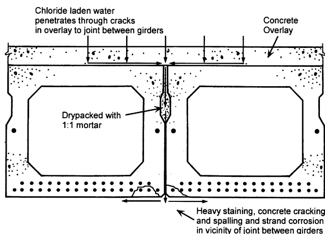
Fig. 7.1—Mechanism for moisture and chloride penetration through concrete overlay in precast, pretensioned box girders (adapted from Novokschenov 1989b).
