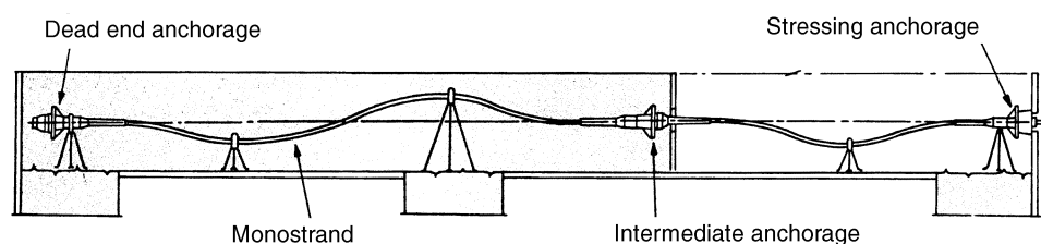
Fig. 4.3—Typical monostrand post-tensioning system components (VSL post-tensioning).
