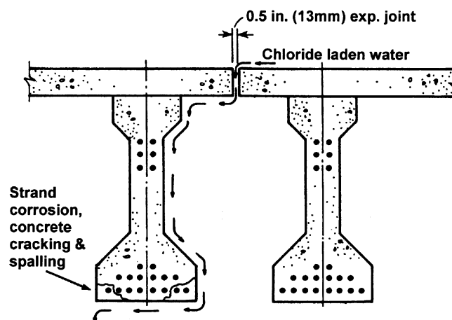
Fig. 7.2—Mechanism for moisture and chloride penetration at longitudinal expansion joints in precast I-girder bridges (adapted from Novokschenov 1989b).
