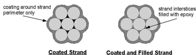
Fig. 4.1—Epoxy-coated strand types.
