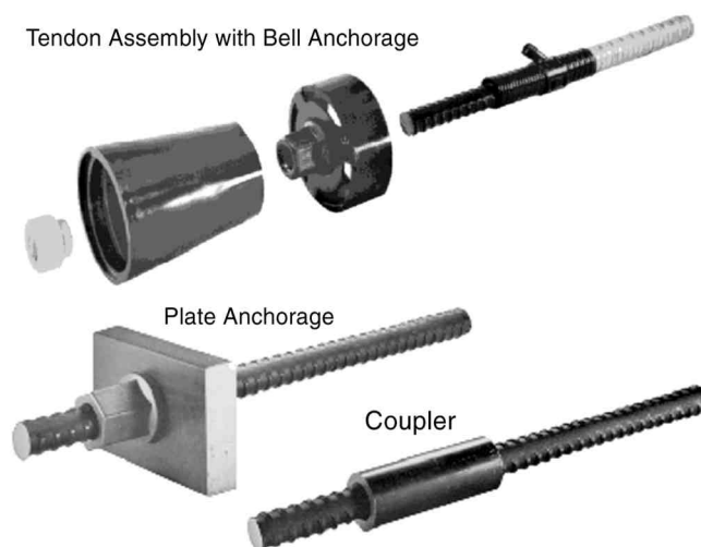
Fig. 4.6—Threadbar post-tensioning system anchorage details (Dywidag International).
