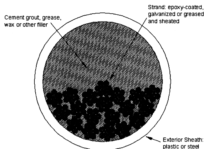
Fig. 4.10—External post-tensioning tendon corrosion protection cross section shown at tendon high point.
