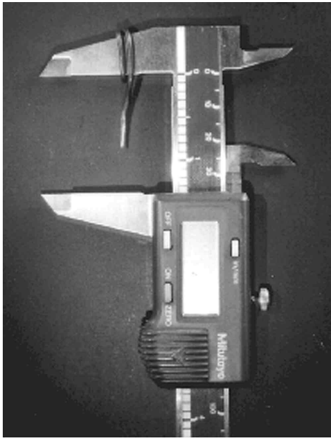
Fig. 5.4—Probe used to estimate pitting depths.
