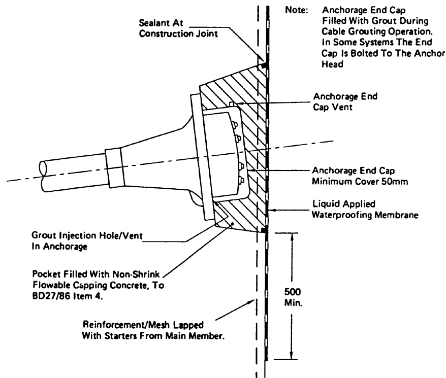
Fig. 4.8—Multilayer corrosion protection for buried post-tensioning anchorages (dimensions in mm; 1 in. = 25.4 mm) (The Concrete Society 1996).
