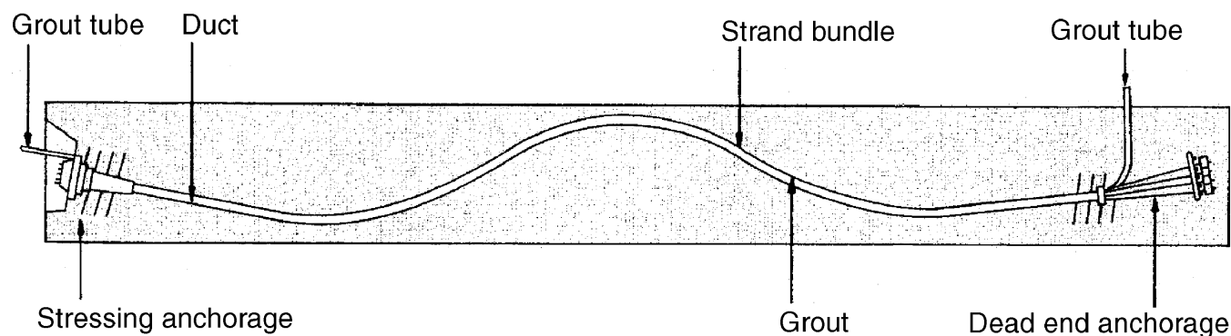
Fig. 4.7—Typical multistrand post-tensioning system components (VSL post-tensioning).
