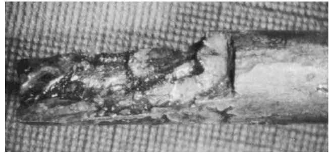
Fig. 5.5—Brittle wire fracture.
